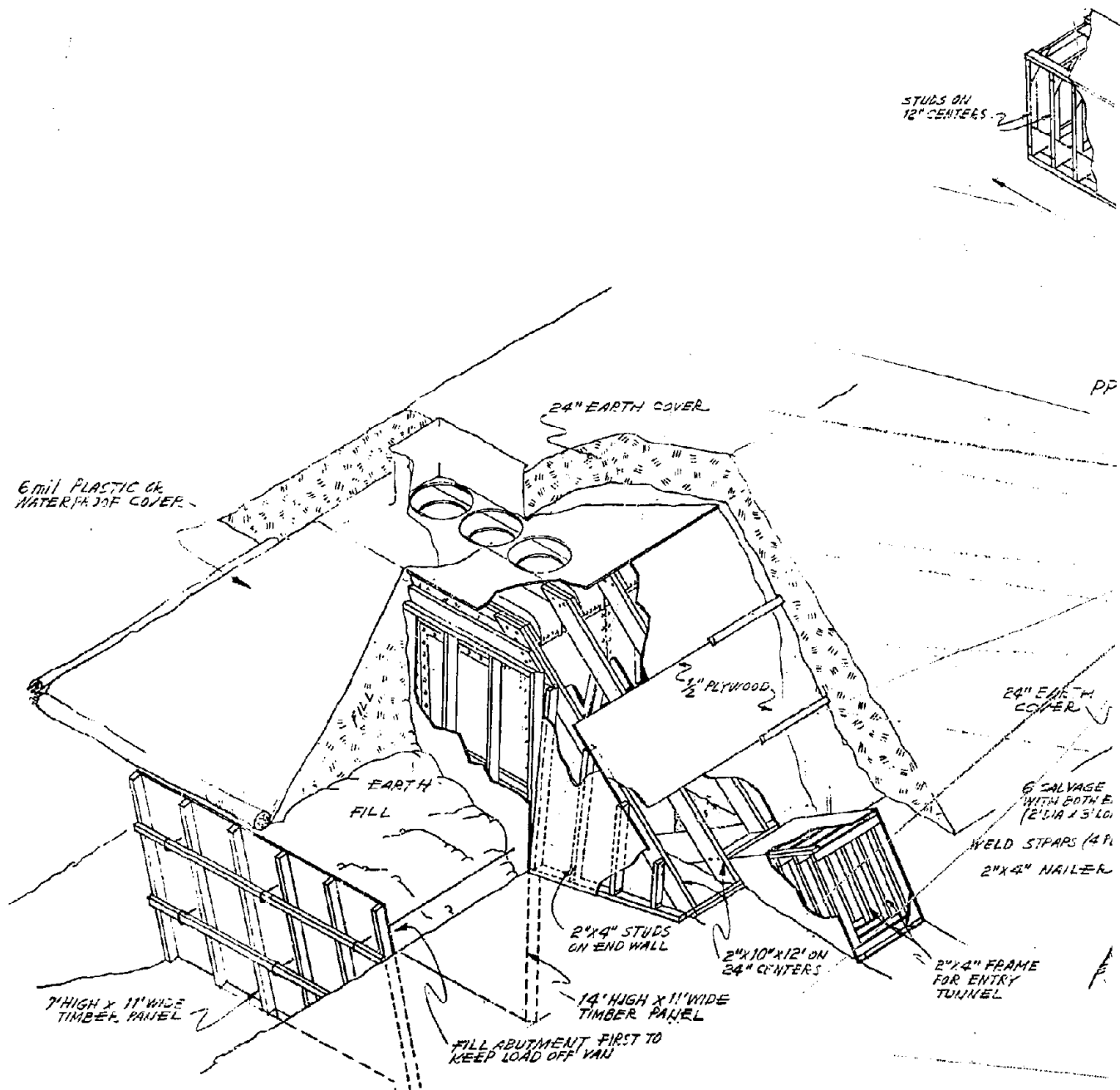
PICTORIAL VIEW OF FRAMING AT END OF VAN SHELTER
